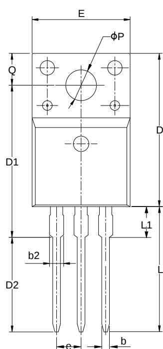
TO-220FJD-3L
