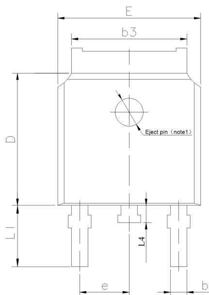
TO-252-2L
