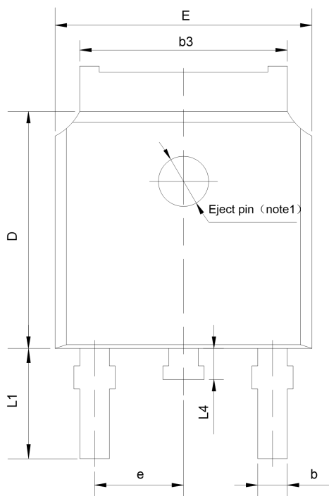
TO-252-2L
