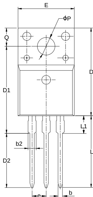
TO-220FJD-3L
