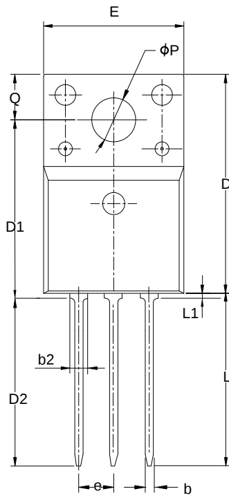
TO-220FJH-3L
