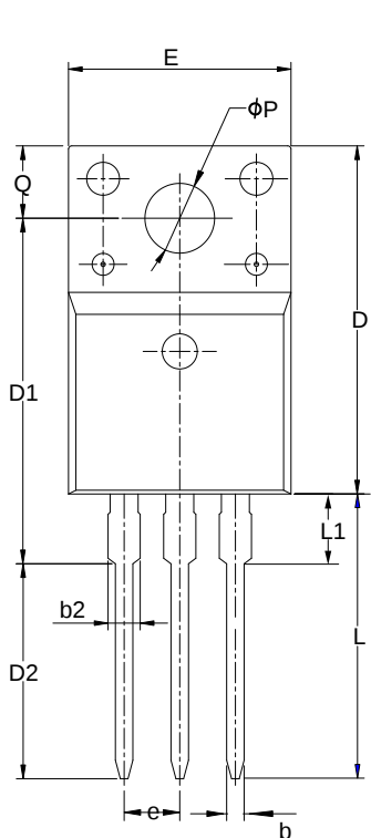
TO-220F-3L
