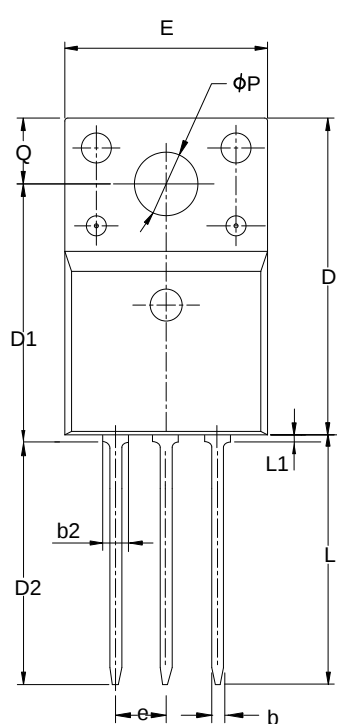
TO-220FJD-3L
